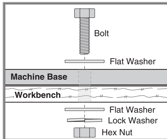
Figure 2. Example of a through mount.
