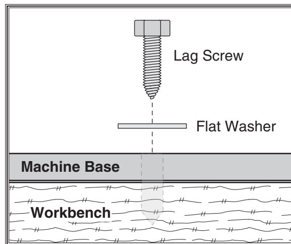
Figure 3. Example of a direct mount.
